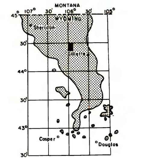
MAP SHOWING LOCATION OF THE ECHETA QUADRANGLE AND THE POWDER RIVER BASIN KNOWN RECOVERABLE COAL RESOURCE AREA (STIPPLED), WYOMING
