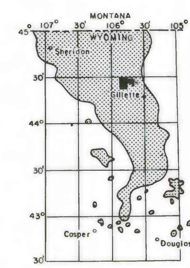
MAP SHOWING LOCATION OF THE TWENTYMILE BUTTE QUADRANGLE AND THE POWDER RIVER BASIN KNOWN RECOVERABLE COAL RESOURCE AREA (STIPPLED), WYOMING
