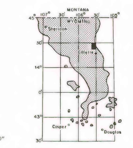
MAP SHOWING LOCATION OF THE RAWHIDE SCHOOL QUADRANGLE AND THE POWDER RIVER BASIN AND KNOWN RECOVERABLE COAL RESOURCE AREA (STIPPLED), WYOMING
