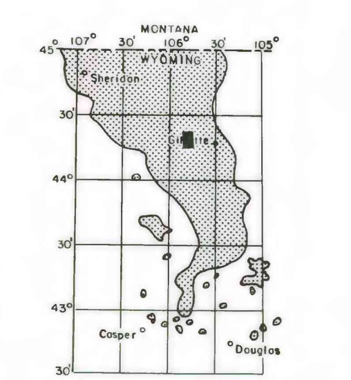
MAP SHOWING LOCATION OF THE JEFFERS DRAW QUADRANGLE AND THE POWDER RIVER BASIN KNOWN RECOVERABLE COAL RESOURCE AREA (STIPPLED), WYOMING
