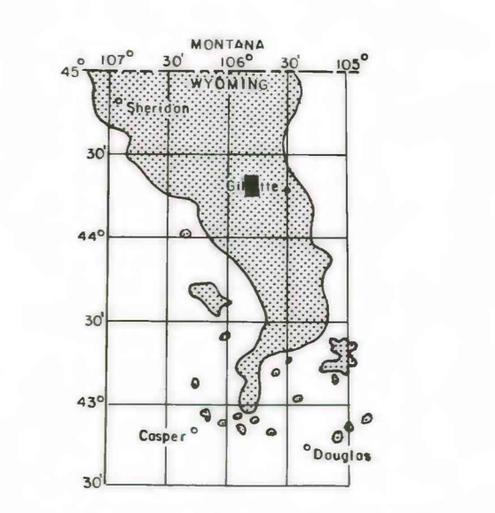
MAP SHOWING LOCATION OF THE JEFFERS DRAW QUADRANGLE AND THE POWDER RIVER BASIN KNOWN RECOVERABLE COAL RESOURCE AREA (STIPPLED), WYOMING
