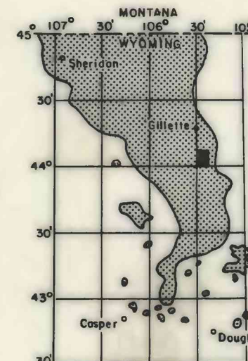
MAP SHOWING LOCATION OF THE GAP SW QUADRANGLE AND THE POWDER RIVER BASIN KNOWN RECOVERABLE COAL RESOURCE AREA (STIPPLED), WYOMING
