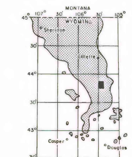
MAP SHOWING LOCATION OF THE REJO JUNCTION QUADRANGLE AND THE POWDER RIVER BASIN KNOWN RECOVERABLE COAL RESOURCE AREA (STIPPLED), WYOMING
