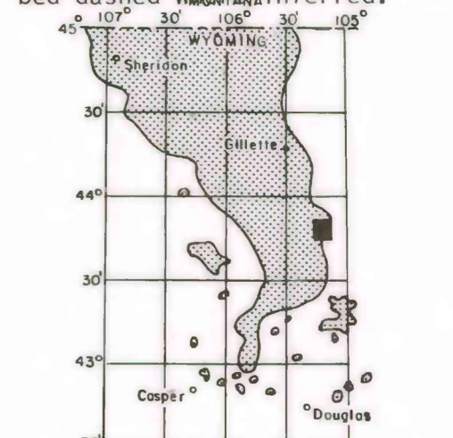
MAP SHOWING LOCATION OF THE OPEN A RANCH QUADRANGLE AND THE POWDER RIVER BASIN KNOWN RECOVERABLE COAL RESOURCE AREA (STIPPLED), WYOMING
