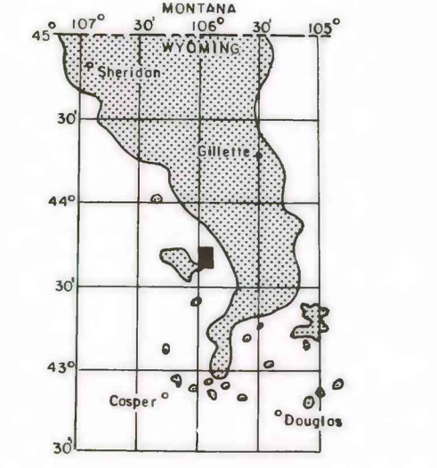
MAP SHOWING LOCATION OF THE ROLLING PIN RANCH QUADRANGLE AND THE POWDER RIVER BASIN KNOWN RECOVERABLE COAL RESOURCE AREA (STIPPLED), WYOMING
