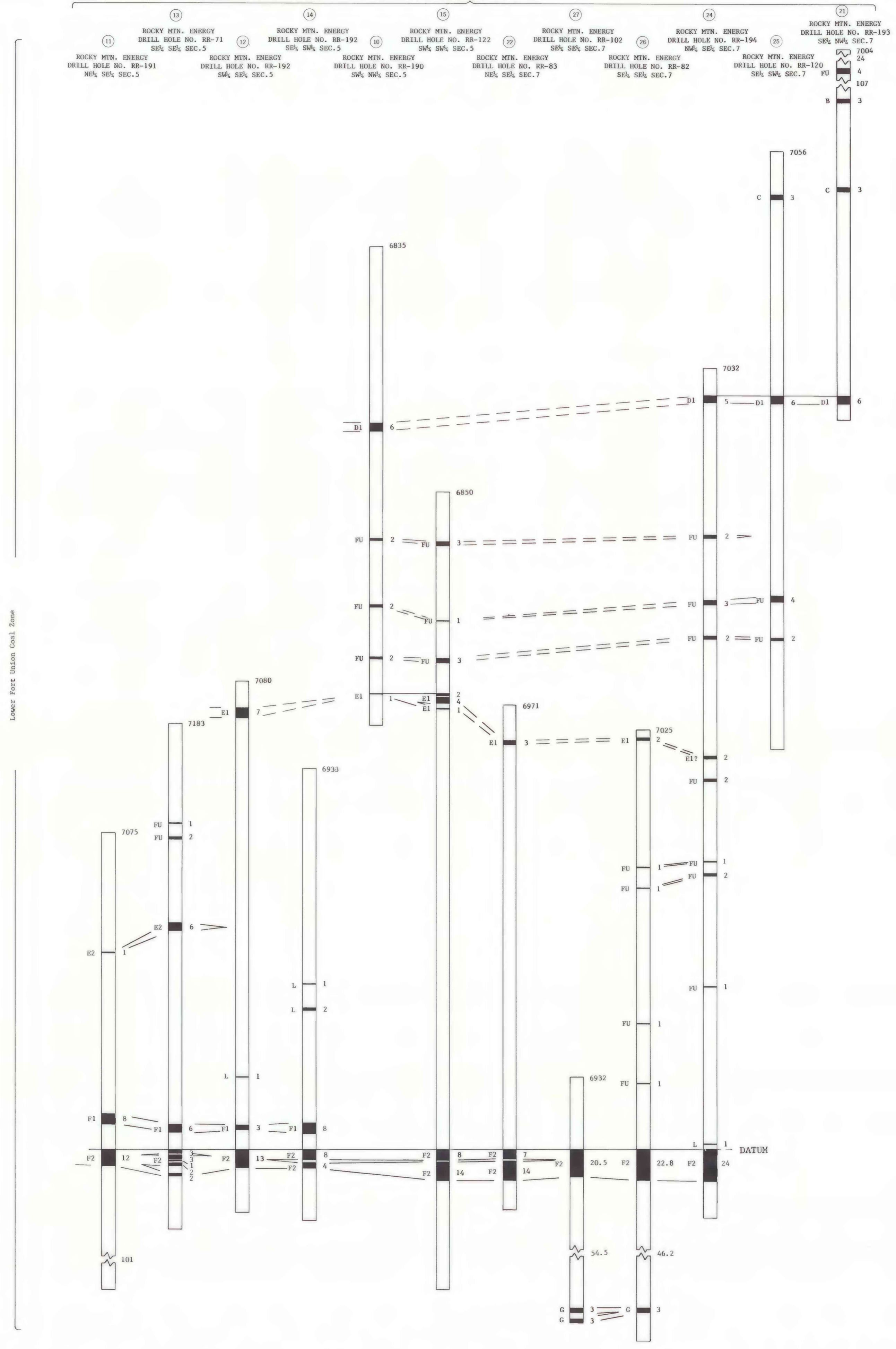
COAL RESOURCE OCCURRENCE MAP OF THE RINER QUADRANGLE, SWEETWATER AND CARBON COUNTIES, WYOMING BY DAMES & MOORE 1979
