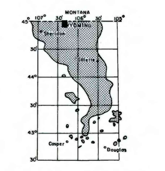
MAP SHOWING LOCATION OF THE BOX ELDER DRAW QUADRANGLE AND THE POWDER RIVER BASIN KNOWN RECOVERABLE COAL RESOURCE AREA (STIPPLED), WYOMING AND MONTANA
