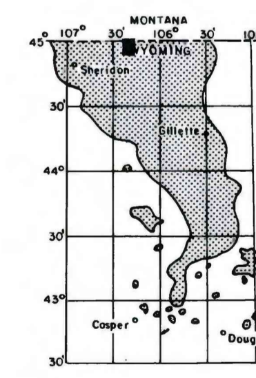
MAP SHOWING LOCATION OF THE BOX ELDER DRAW QUADRANGLE AND THE POWDER RIVER BASIN KNOWN RECOVERABLE COAL RESOURCE AREA (STIPPLED), WYOMING AND MONTANA
