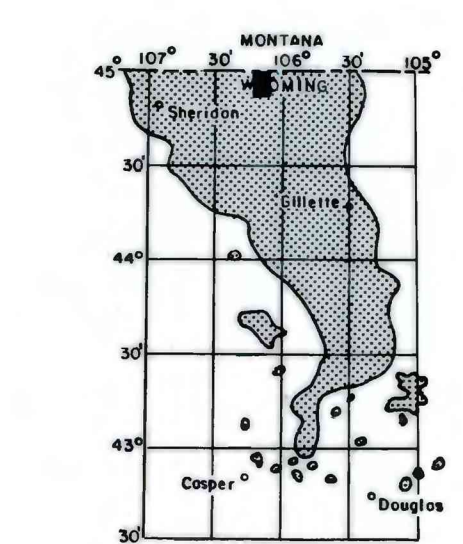
MAP SHOWING LOCATION OF THE CABIN CREEK NW QUADRANGLE AND THE POWDER RIVER BASIN KNOWN RECOVERABLE COAL RESOURCE AREA (STIPPLED), WYOMING AND MONTANA
