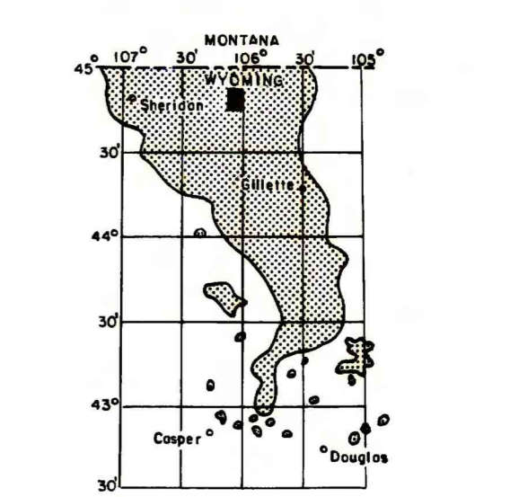
MAP SHOWING LOCATION OF THE CABIN CREEK SE QUADRANGLE AND THE POWDER RIVER BASIN KNOWN RECOVERABLE COAL RESOURCE AREA (STIPPLED), WYOMING
