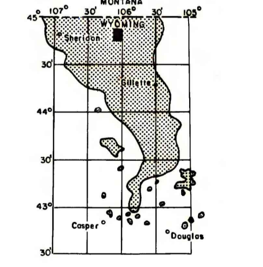
MAP SHOWING LOCATION OF THE CABIN CREEK SE QUADRANGLE AND THE POWDER RIVER BASIN KNOWN RECOVERABLE COAL RESOURCE AREA (STIPPLED), WYOMING
