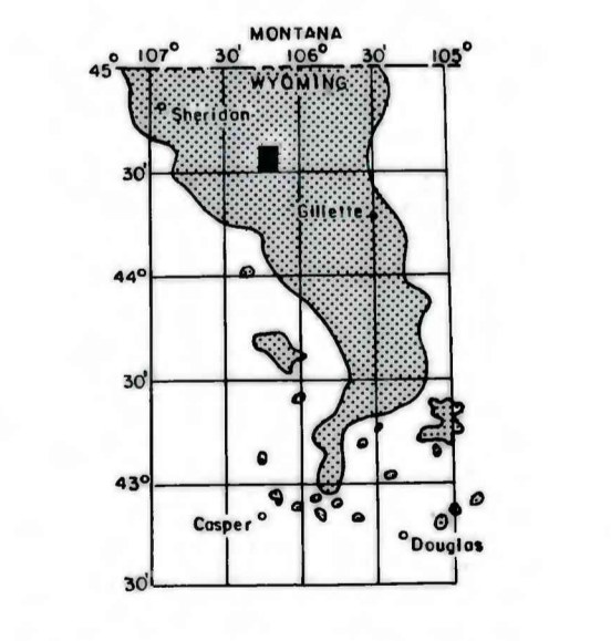
MAP SHOWING LOCATION OF THE JEWELL DRAW QUADRANGLE AND THE POWDER RIVER BASIN KNOWN RECOVERABLE COAL RESOURCE AREA (STIPPLED), WYOMING
