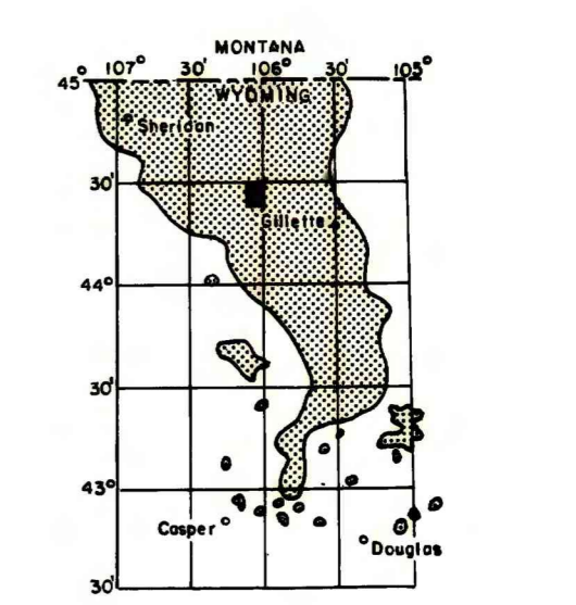
MAP SHOWING LOCATION OF THE LIVINGSTON DRAW QUADRANGLE AND THE POWDER RIVER BASIN KNOWN RECOVERABLE COAL RESOURCE AREA (STIPPLED), WYOMING
