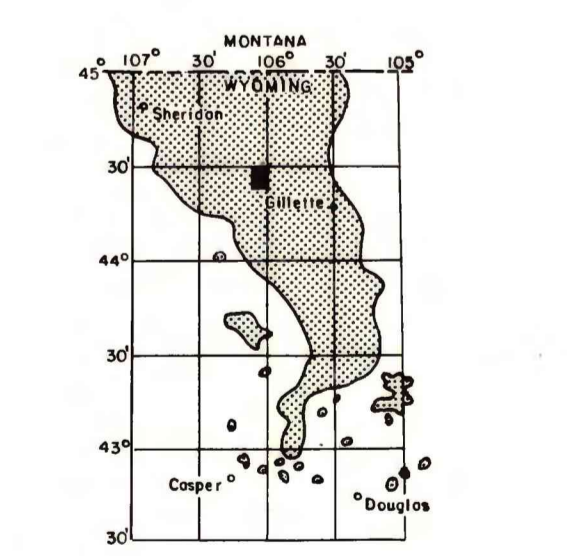
MAP SHOWING LOCATION OF THE LIVINGSTON DRAW QUADRANGLE AND THE POWDER RIVER BASIN KNOWN RECOVERABLE COAL RESOURCE AREA (STIPPLED), WYOMING
