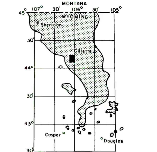
MAP SHOWING LOCATION OF THE LASKIE DRAW QUADRANGLE AND THE POWDER RIVER BASIN KNOWN RECOVERABLE COAL RESOURCE AREA (STIPPLED), WYOMING
