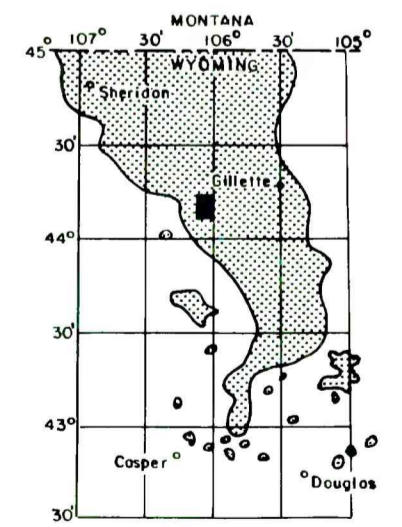
MAP SHOWING LOCATION OF THE LASKIE DRAW QUADRANGLE AND THE POWER RIVER BASIN KNOWN RECOVERABLE COAL RESOURCE AREA (STIPPLED), WYOMING
