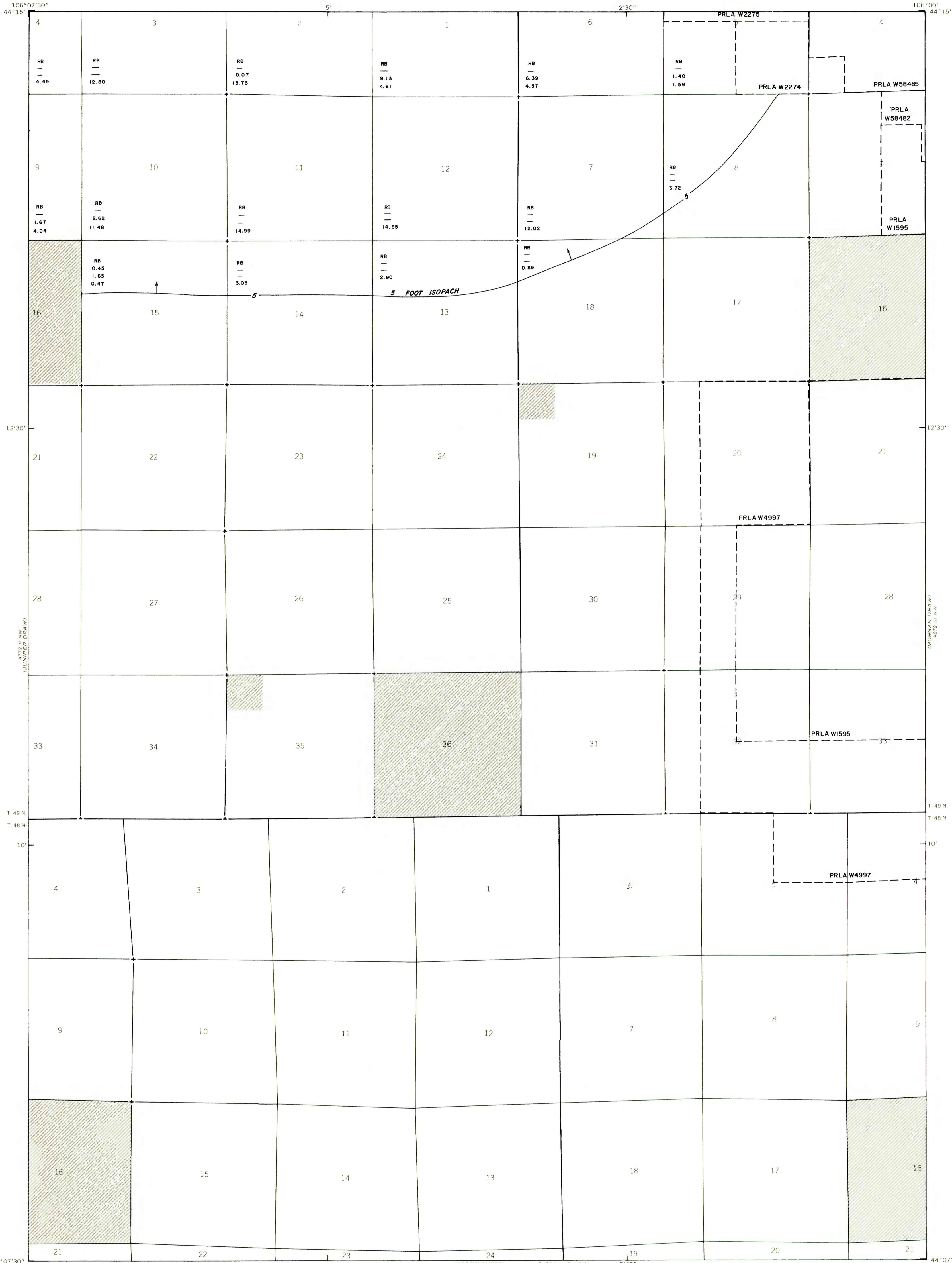
MAP SHOWING LOCATION OF THE LASKIE DRAW QUADRANGLE AND THE POWER RIVER BASIN KNOWN RECOVERABLE COAL RESOURCE AREA (STIPPLED), WYOMING
