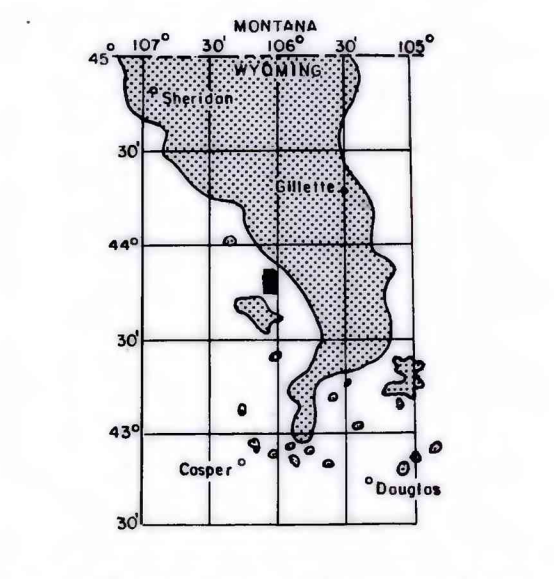
MAP SHOWING LOCATION OF THE FORT RENO SE QUADRANGLE AND THE POWDER RIVER BASIN KNOWN RECOVERABLE COAL RESOURCE AREA (STIPPLED), WYOMING
