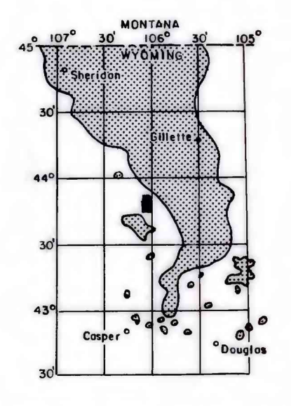
MAP SHOWING LOCATION OF THE FORT RENO SE QUADRANGLE AND THE POWDER RIVER BASIN KNOWN RECOVERABLE COAL RESOURCE AREA (STIPPLED), WYOMING
