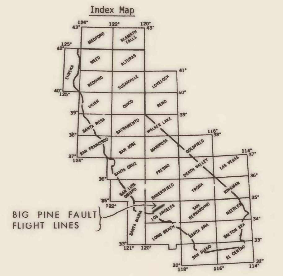
Route of flight lines through 1° x 2° quadrangles (scale 1:250,000) along the Big Pine fault.
