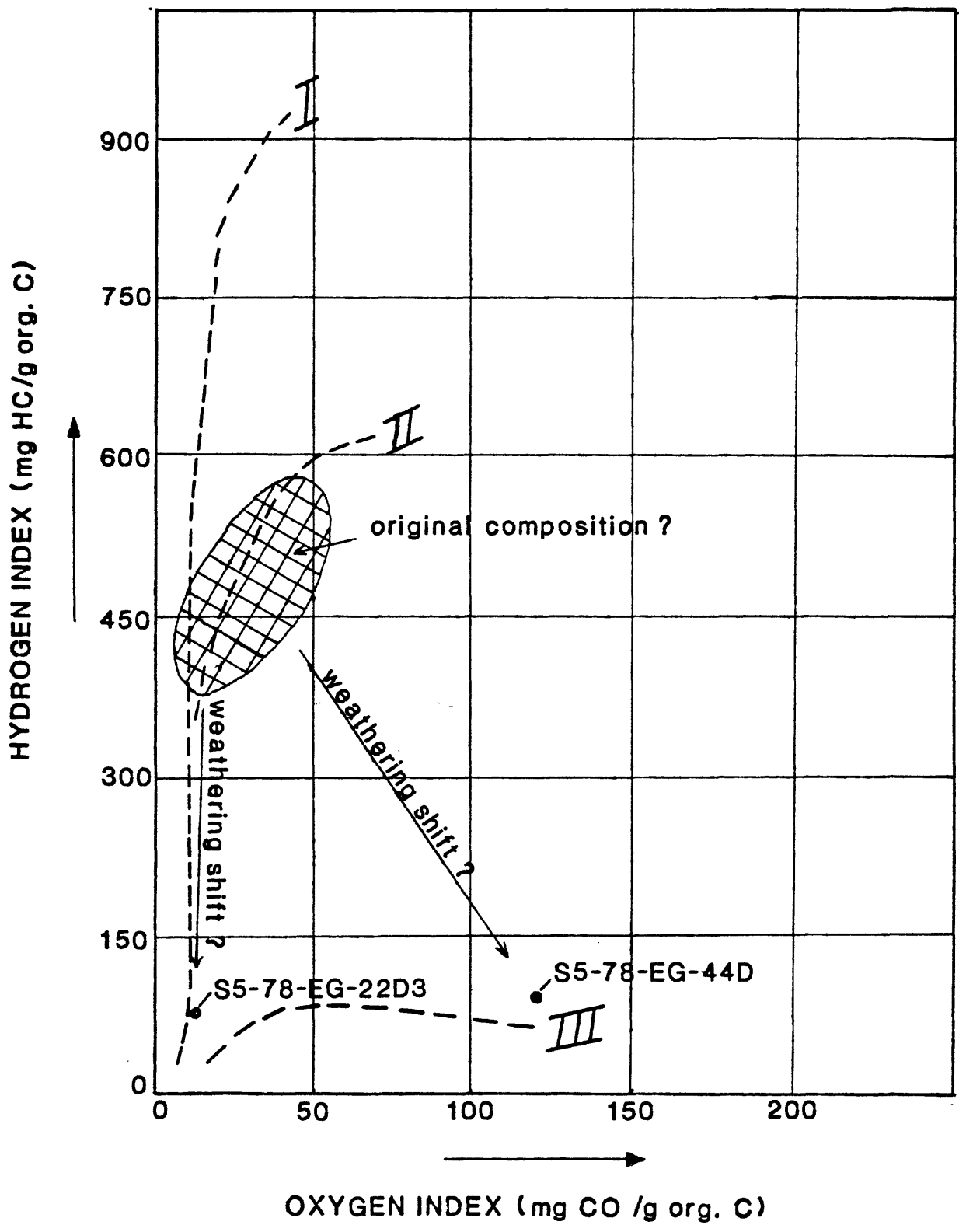
Figure 3.--Classification of source rock type for the 1978 samples using hydrogen and oxygen indices (Espitalié and others, 1977). The evolutionary trends of kerogen derived mainly from aquatic organisms (Type I), herbaceous plant material (Type II), and woody or coaly plant material (Type III) are shown by heavy dashed lines. Circled field indicates possible original composition, and arrows indicate possible shifts due to weathering of the pyrolysis response of the 1978 samples.
