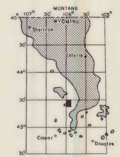
MAP SHOWING LOCATION OF THE NW¼ ROSS 15' QUADRANGLE AND THE POWDER RIVER BASIN KNOWN RECOVERABLE COAL RESOURCE AREA (STIPPLED), WYOMING
