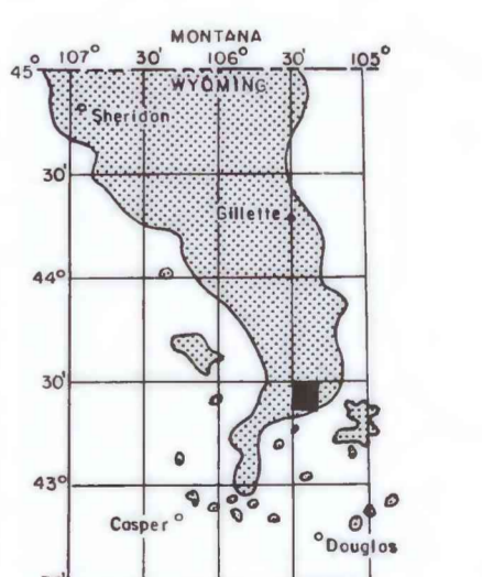
MAP SHOWING LOCATION OF THE NW¼ BETTY RESERVOIR 15' QUADRANGLE AND THE POWDER RIVER BASIN KNOWN RECOVERABLE COAL RESOURCE AREA (STIPPLED), WYOMING
