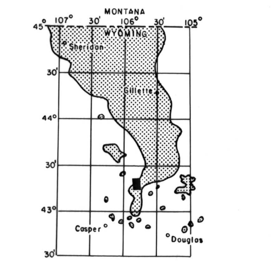
MAP SHOWING LOCATION OF THE SE¼ ROSS 15' QUADRANGLE AND THE POWDER RIVER BASIN KNOWN RECOVERABLE COAL RESOURCE AREA (STIPPLED), WYOMING
