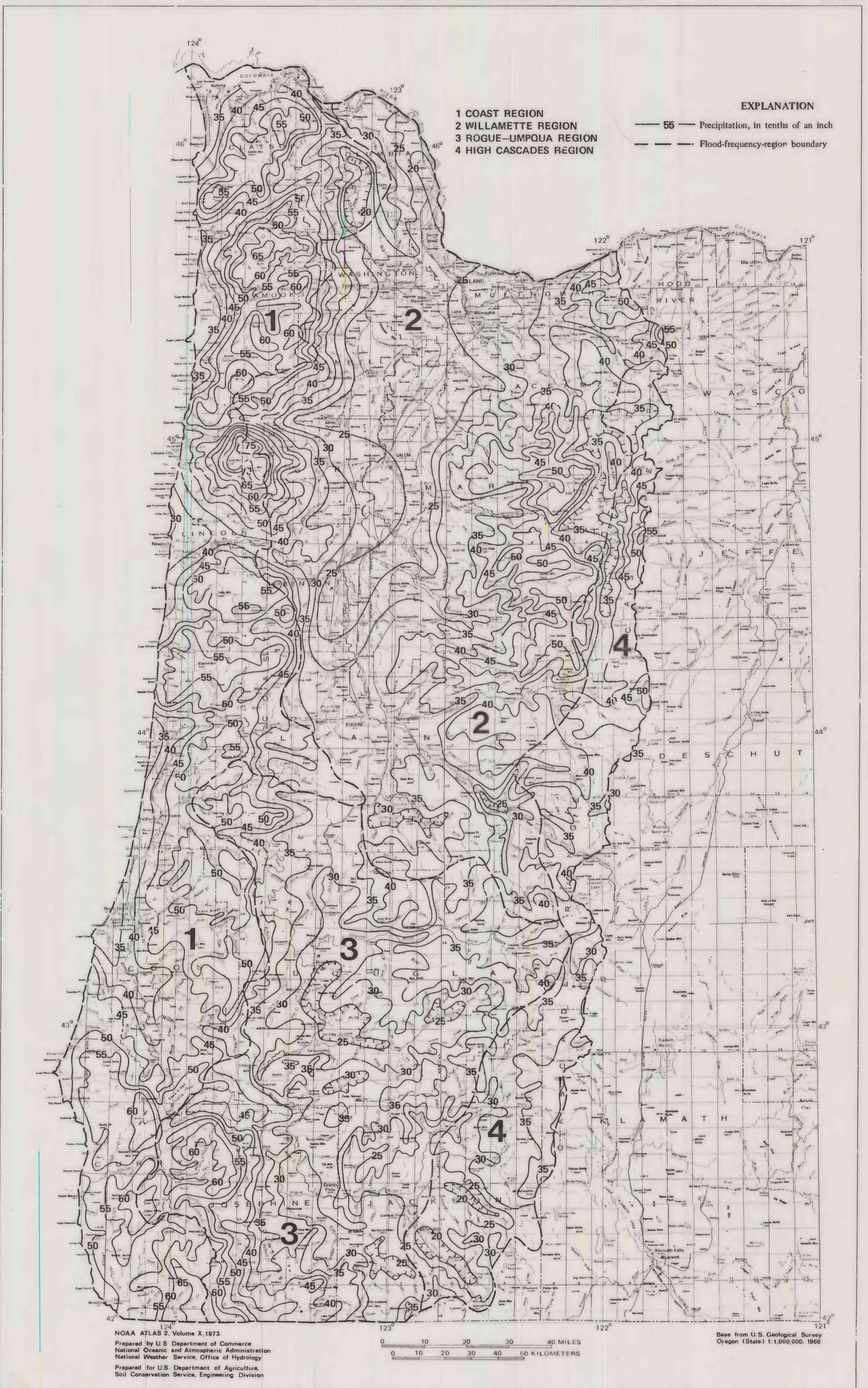
PLATE 2.—ISOPLUVIALS OF 2-YR, 24-HOUR PRECIPITATION IN TENTHS OF AN INCH FOR WESTERN OREGON
