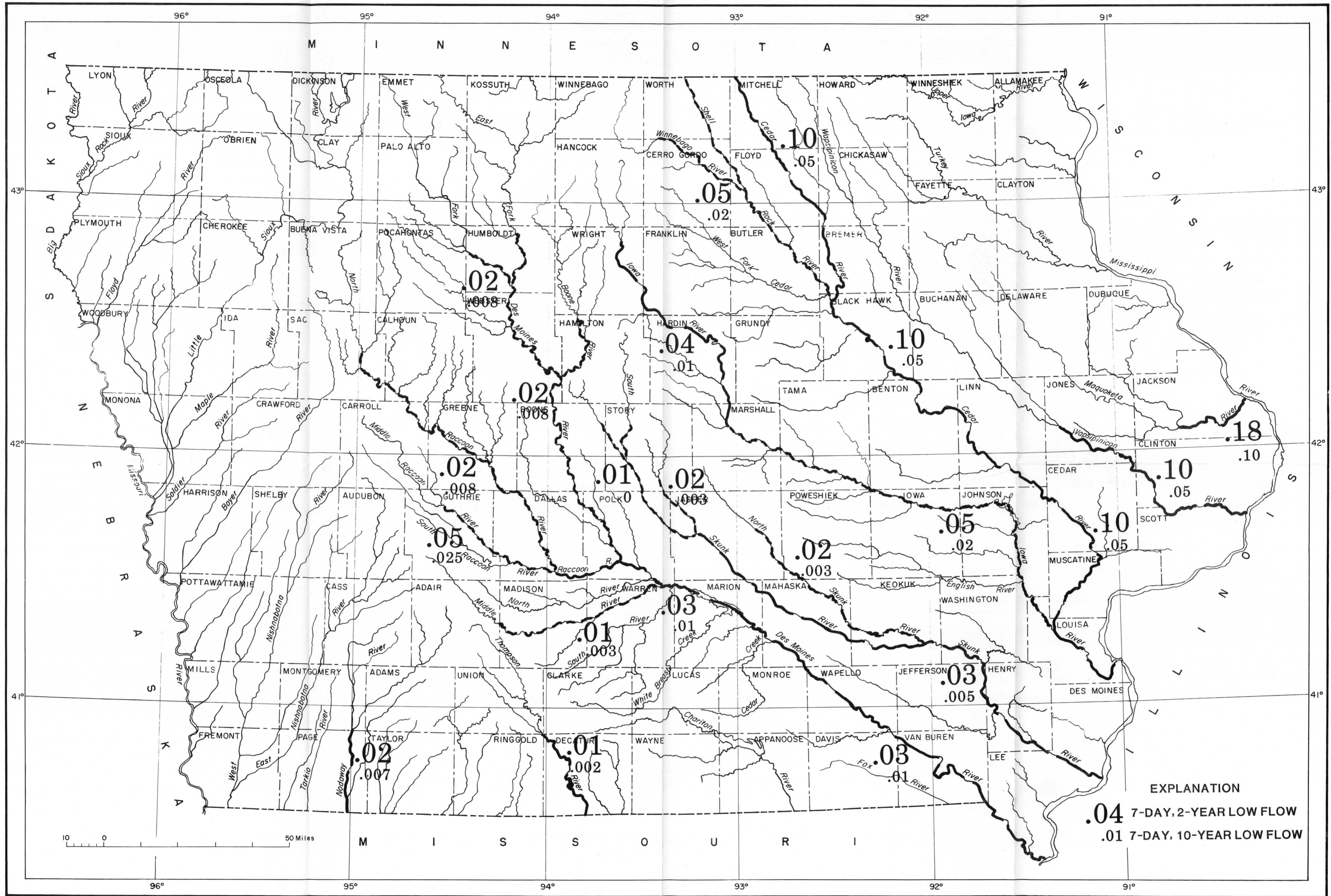
Plate 3. 7-day Q2 and 7-day Q10 low flow, in cubic feet per second, per square mile, for main stems of selected streams.
