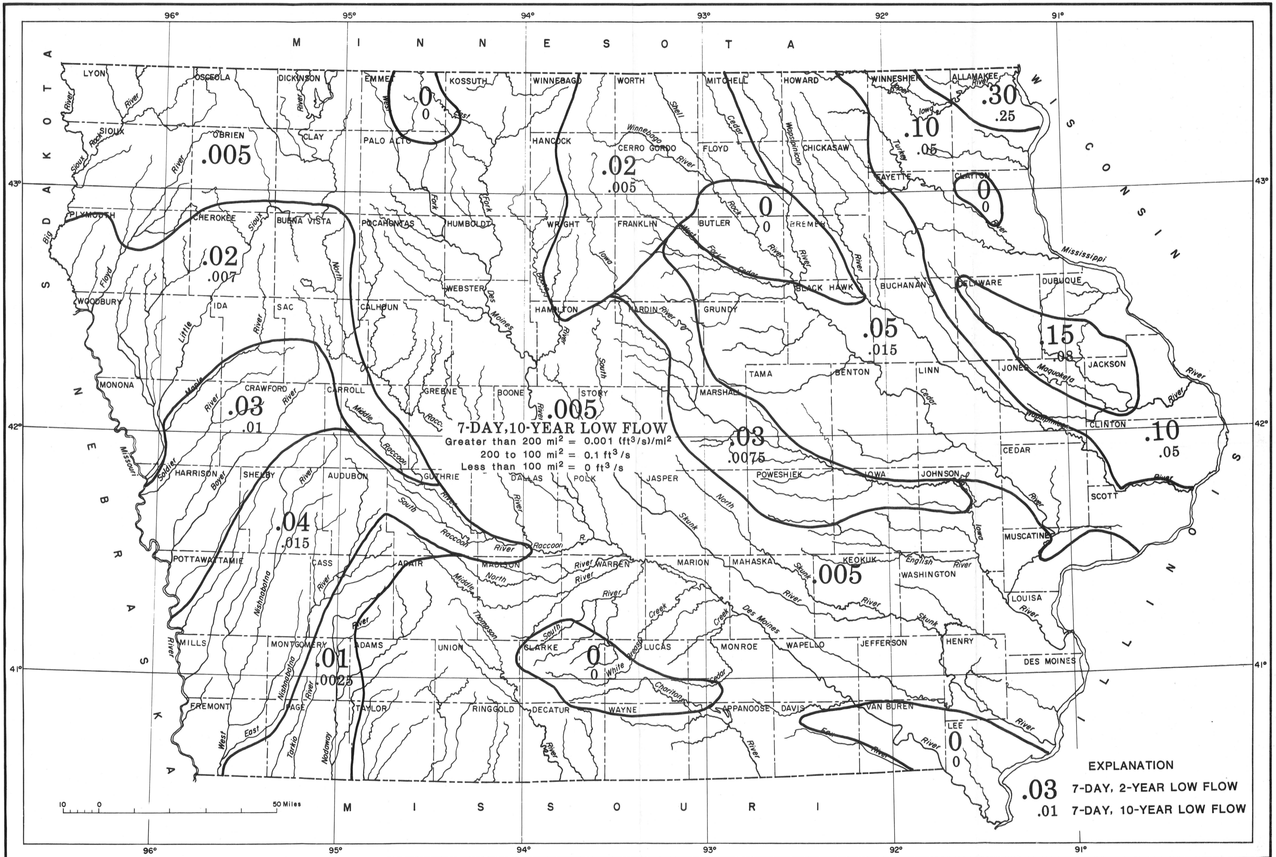
Plate 4. 7-day Q2 and 7-day Q10 low flow, in cubic feet per second per square mile, for all stream points other than main stems shown in Plate 3.
