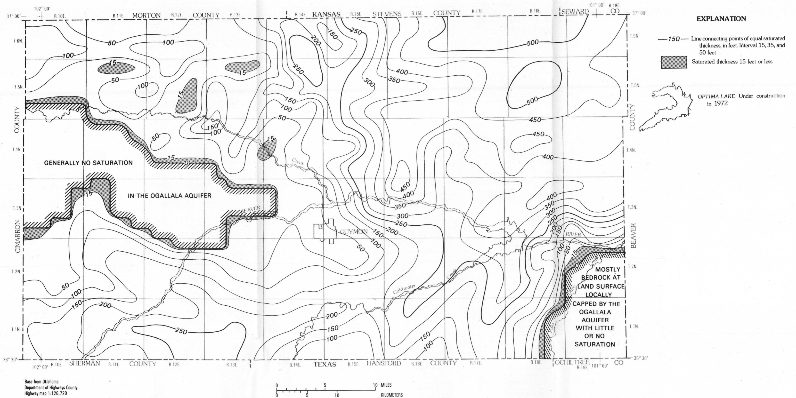
MAP SHOWING SATURATED THICKNESS AT THE END OF MODEL SIMULATION TEST 2, FROM 1972 TO 1993, USING THE 1972 PUMPAGE RATE AND DISTRIBUTION, OGALLALA AQUIFER, TEXAS COUNTY, OKLAHOMA.
