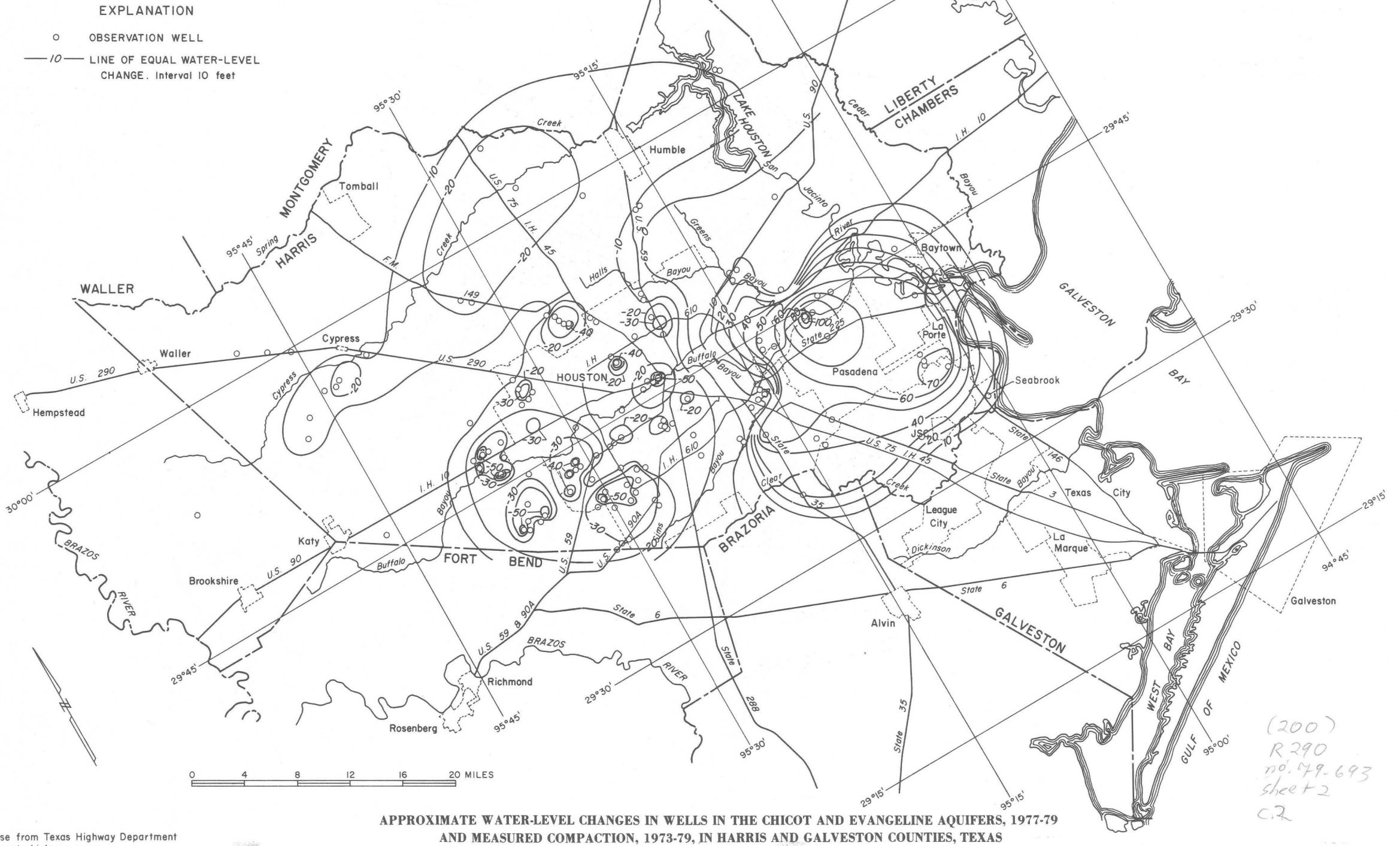
FIGURE 2.—APPROXIMATE WATER-LEVEL CHANGES IN WELLS IN THE EVANGELINE AQUIFER IN HARRIS AND GALVESTON COUNTIES, TEXAS, 1977-79
