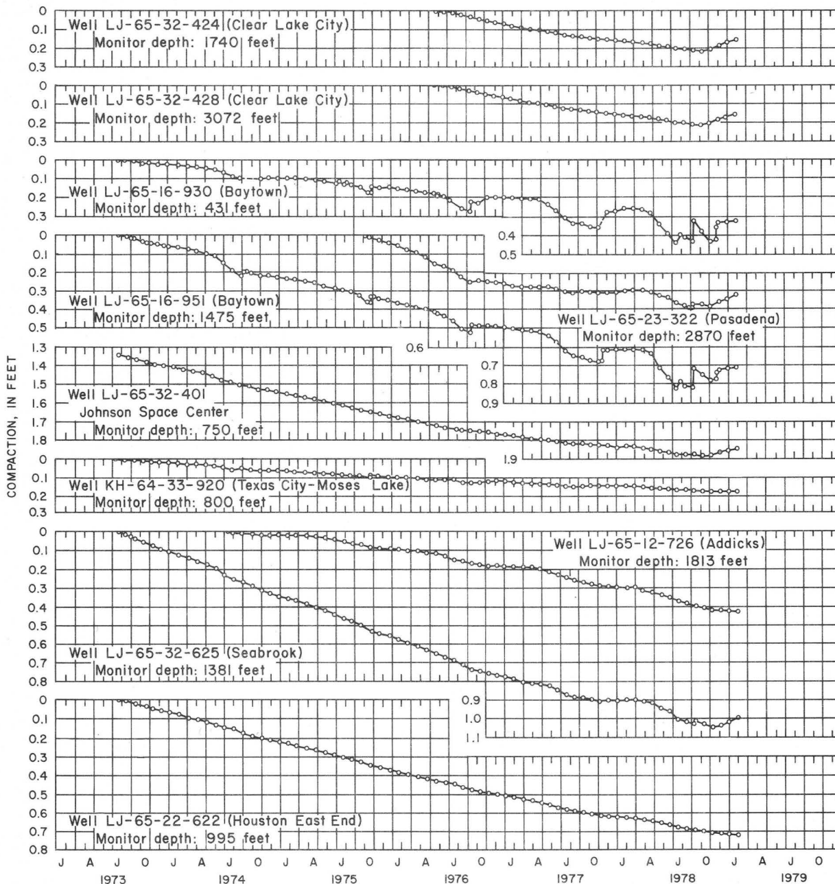
FIGURE 5.-MEASURED COMPACTION IN HARRIS AND GALVESTON COUNTIES, TEXAS, 1973-79
