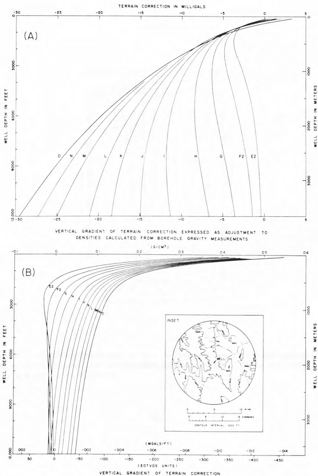
Figure 5. Cumulative terrain corrections (part A) and corresponding vertical gradients of terrain corrections (part B) out through modified Hayford-Bowie zones E2 to O in relation to well depth for the Mountain Fuel Supply Co. Dry Piney Unit 19, 15-27N-114W, Sublette County, Wyoming. Terrain corrections are computed using a density of 2.67 g/cm 3 . Inset shows topography around well out through Hayford-Bowie zone J.
