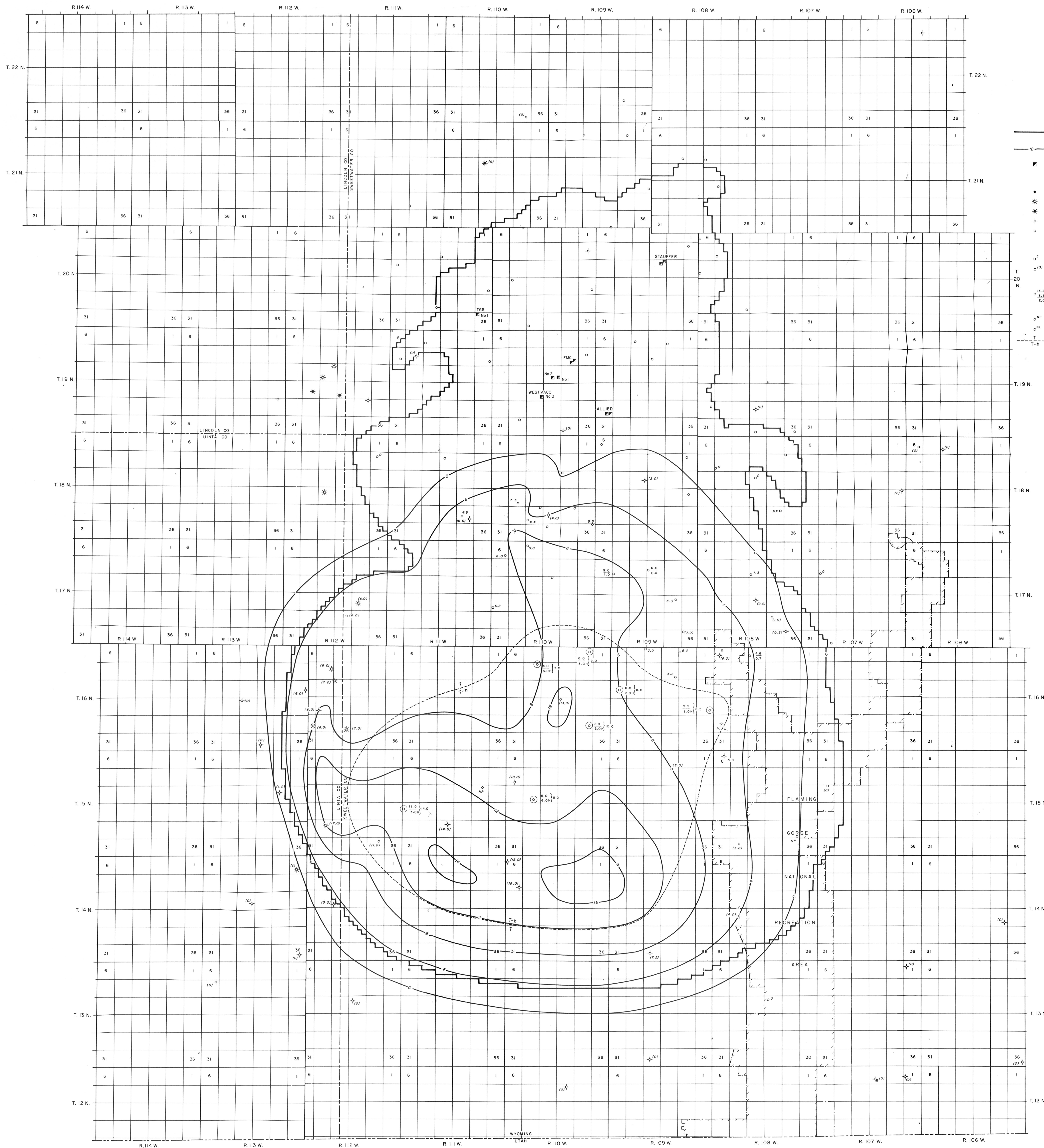
ISOPACH MAP OF NET TRONA AND/OR TRONA-HALITE IN BED 12
