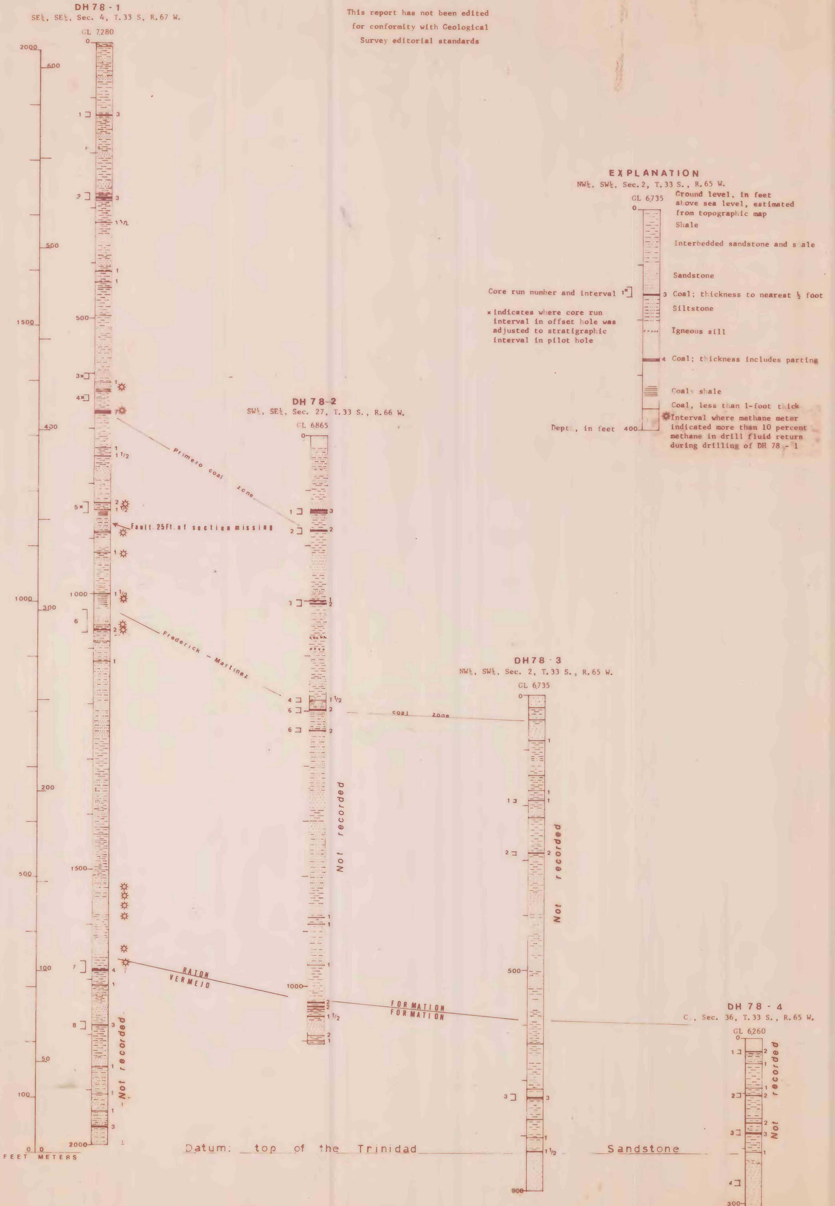
Plate 1. -- LITHOLOGIC LOGS OF U. S. GEOLOGICAL SURVEY DRILL HOLES 78-1, 78-2, 78-3, and 78-4 SHOWING METHANE SOURCES IN DRILL FLUID
