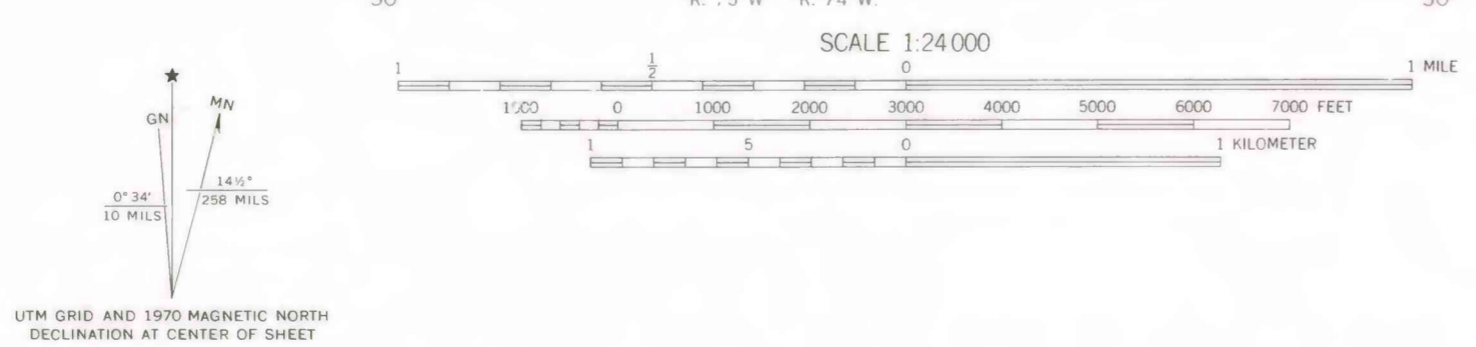
COAL RESOURCE OCCURRENCE MAP OF THE MOORHEAD QUADRANGLE, POWDER RIVER COUNTY, MONTANA, AND CAMPBELL COUNTY, WYOMING BY COLORADO SCHOOL OF MINES RESEARCH INSTITUTE 1979
