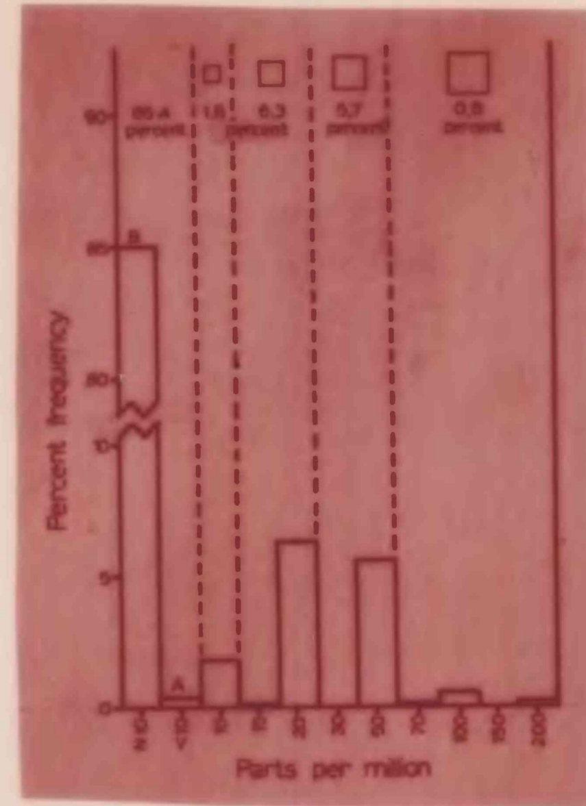
79-837-P Figure 1.--Histogram for tin in 1493 minus-80-mesh stream-sediment samples, Survey Pass 1° x 3° quadrangle, Alaska, showing map symbols corresponding to anomalous concentrations in parts per million, percentage of total samples, and letters corresponding to non-anomalous concentrations in parts per million. N, not detected at values shown; <, detected, but less than value shown. Arithmetic mean, 34; standard deviation, 23; geometric mean, 28; and geometric deviation, 1.9, based on unqualified values within the sample population.
