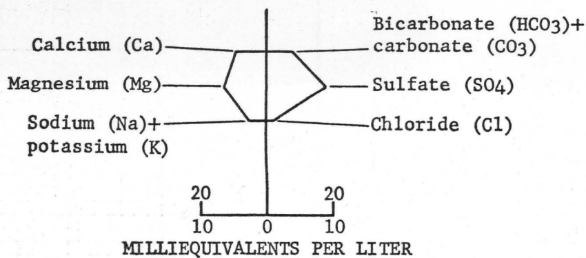
Water-quality diagram (after Stiff, 1951)
