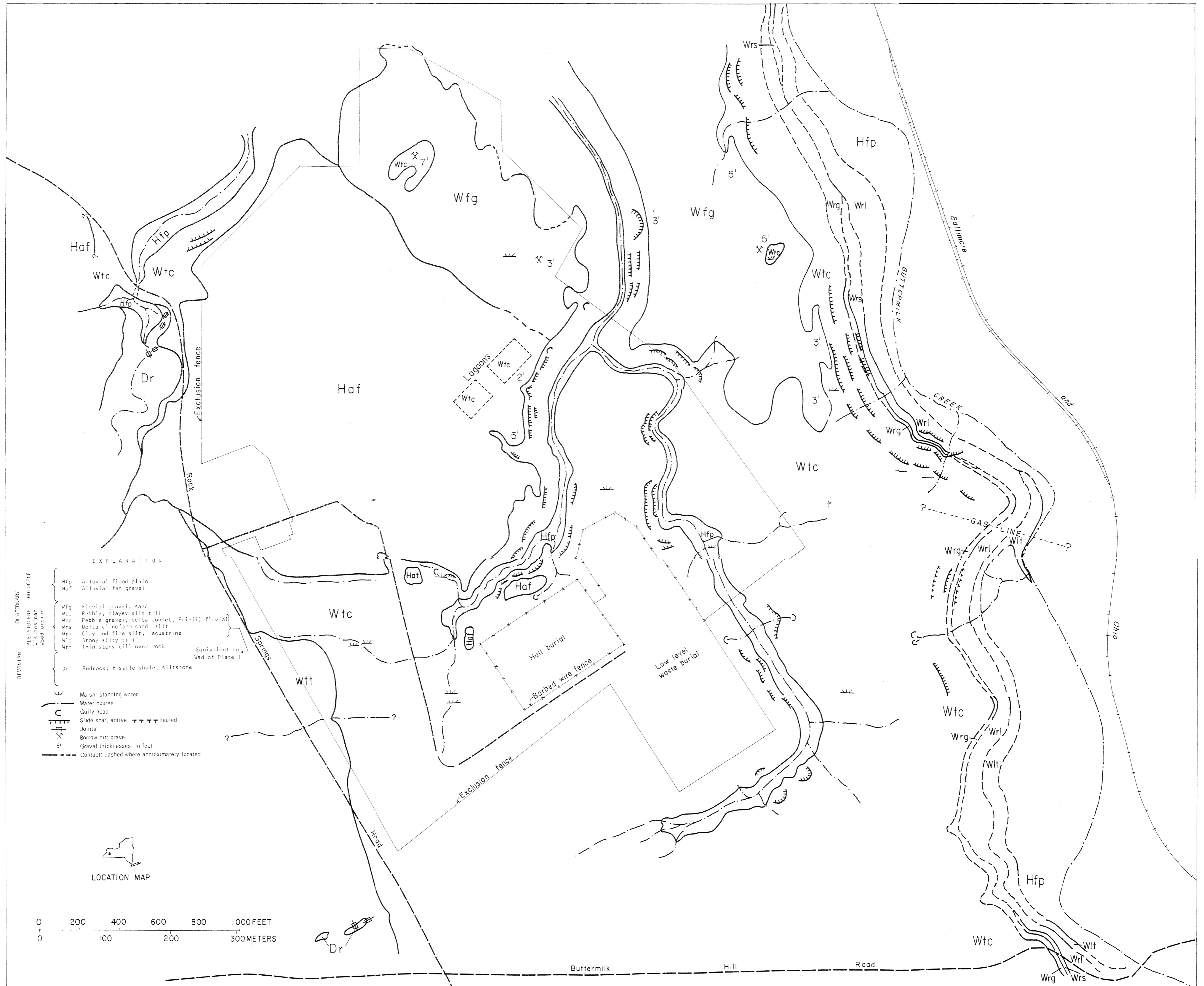
SURFICIAL GEOLOGY OF WESTERN NEW YORK NUCLEAR SERVICE CENTER SPENT-FUEL PROCESSING PLANT, WEST VALLEY, N.Y.
