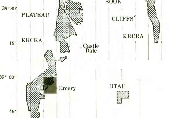
MAP SHOWING LOCATION OF THE EMERY WEST QUADRANGLE (SHADED) AND THE BOOK CLIFFS AND WASATCH PLATEAU KNOWN RECOVERABLE COAL RESOURCE AREAS (STIPPLED), UTAH.
