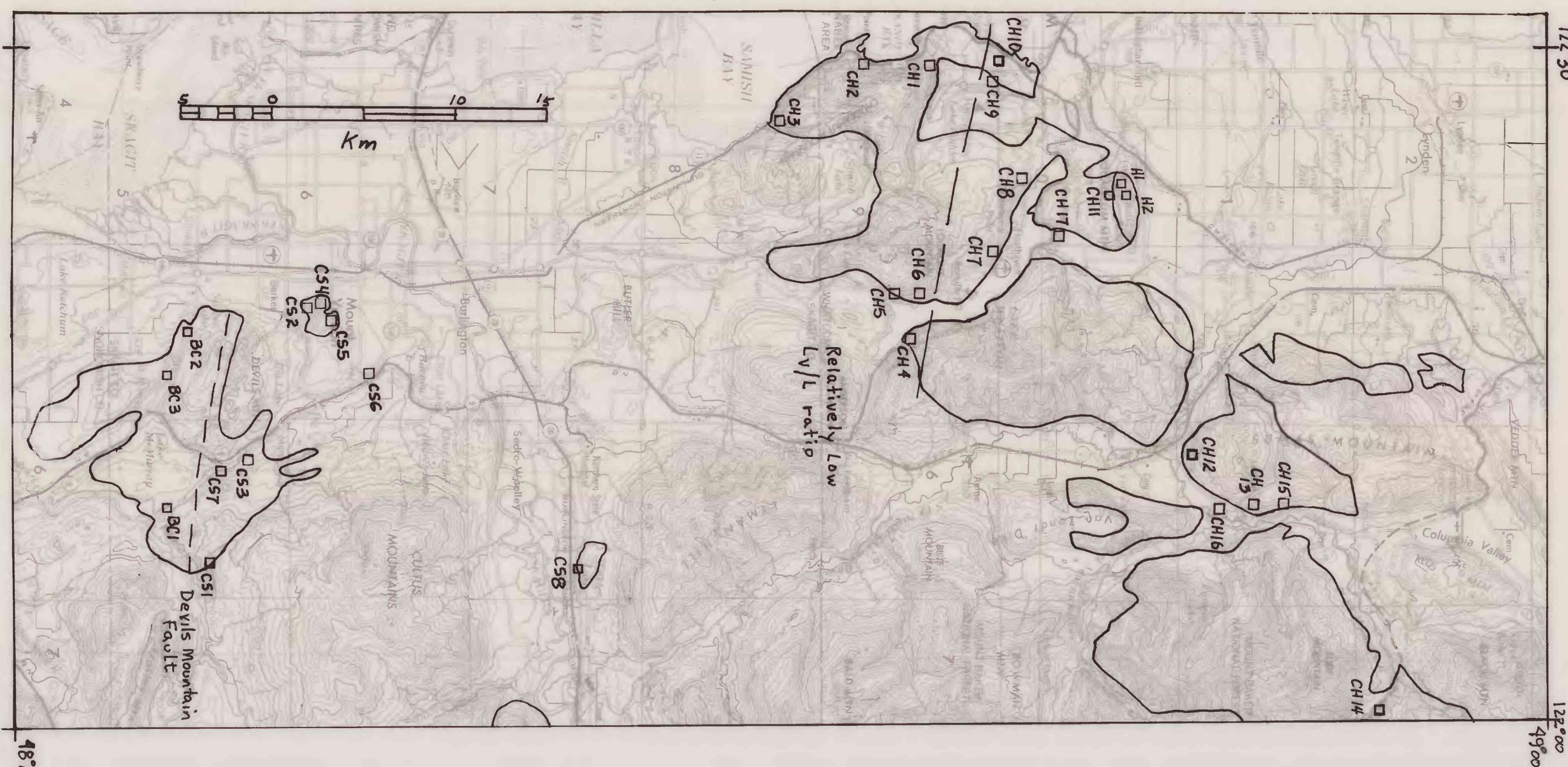
Plate 1 Map showing generalized outcrop patterns and sample localities for Chumstick (CH) and Huntington (H) Formations, rocks of Bolson Creek (BC), and rocks in isolated arkosic bodies (CS), Washington. Also shown: Devils Mountain Fault and a line separating rocks with very low hylt values from other Chumstick samples. Generalized geology after Huntington and others, 1961, and Eastbrook, 1976. Base from U.S.G.S. Victorville Sheet (U.S. revised 1974).
