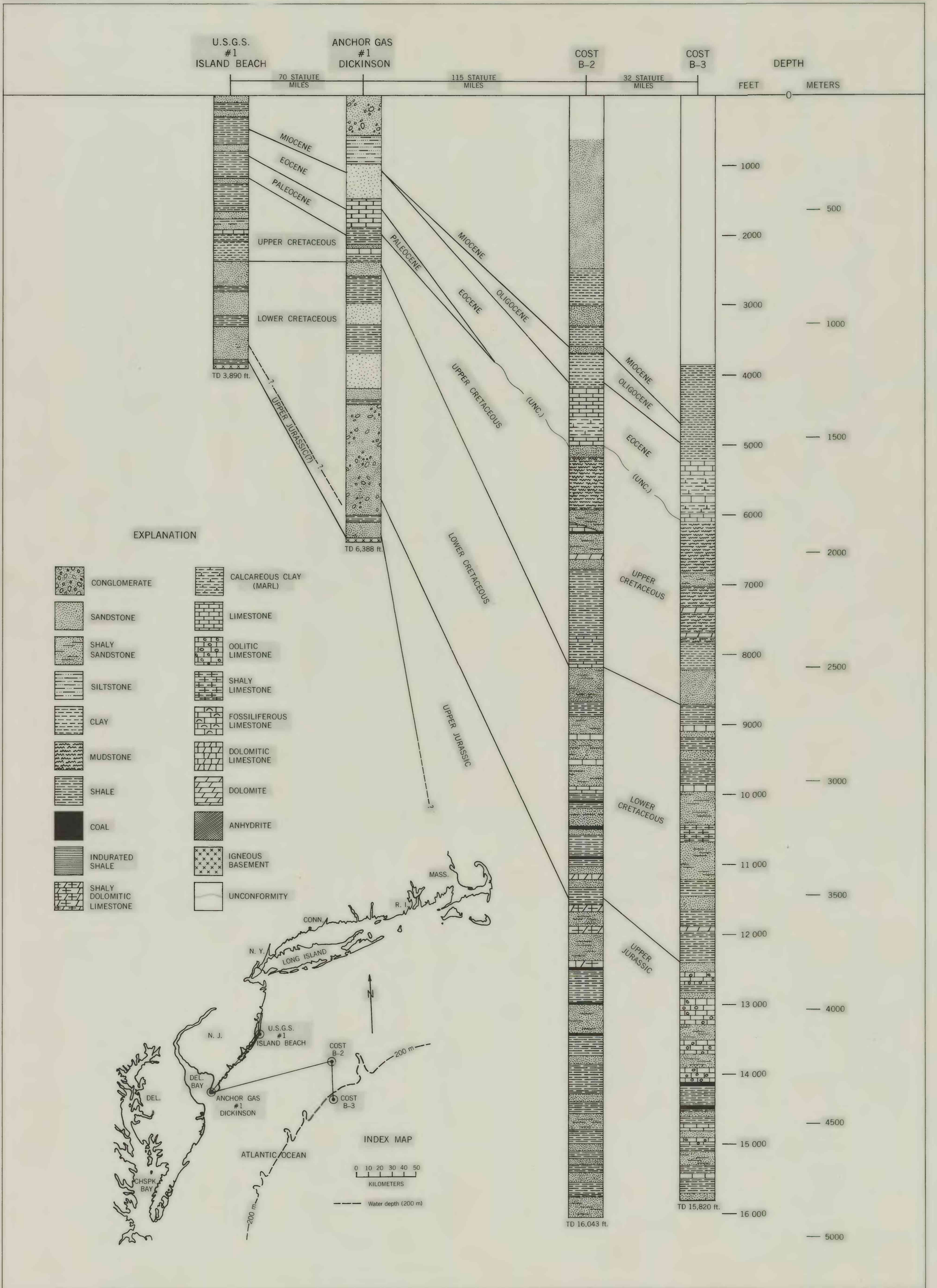
Plate 4. GEOLOGIC CROSS SECTION OF THE MID-ATLANTIC CONTINENTAL SHELF AND COASTAL PLAIN OF NEW JERSEY SHOWING MESOZOIC AND CENOZOIC ROCKS
