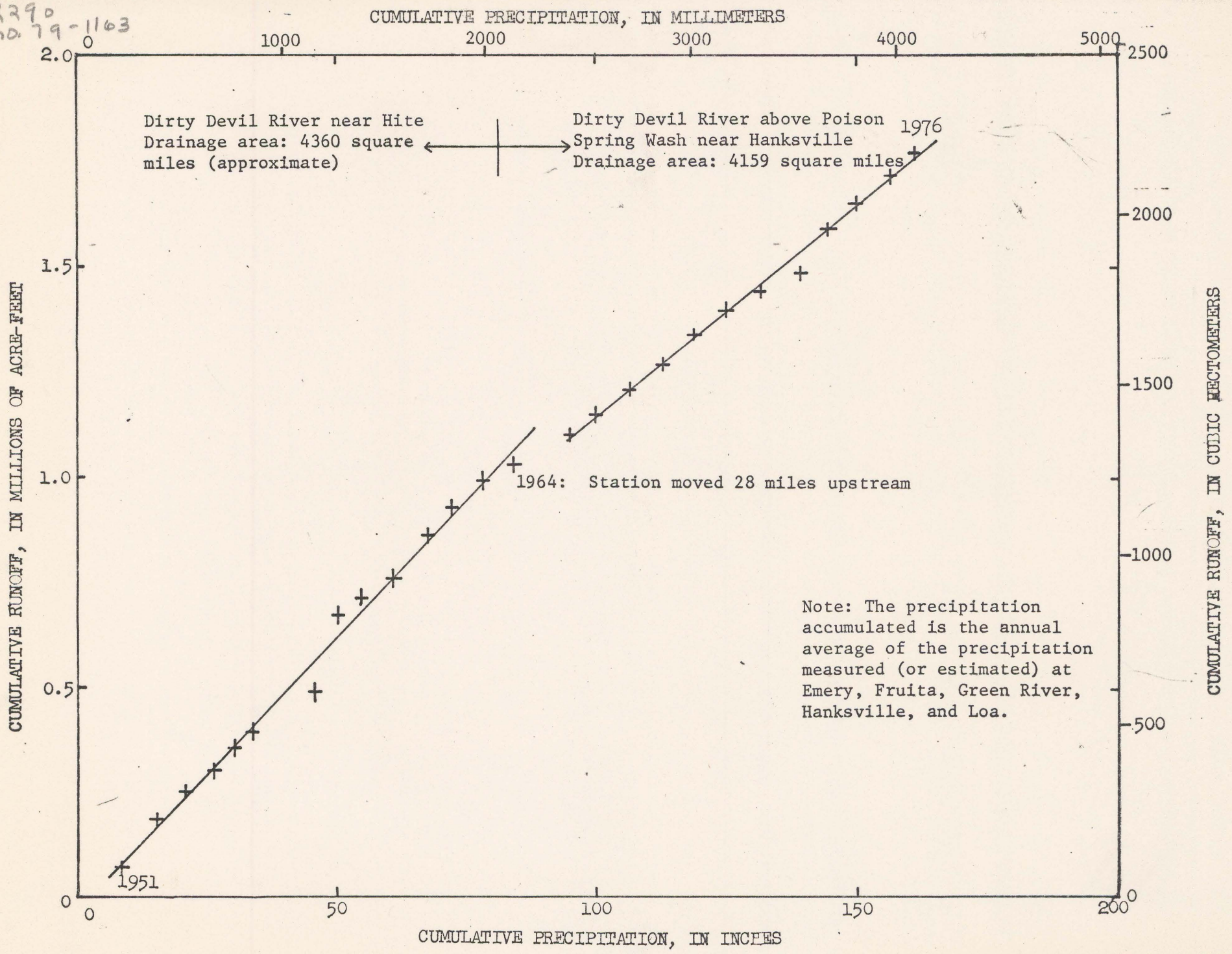
Figure 16.--Runoff at station 3335 versus precipitation in and near the Dirty Devil River basin.
