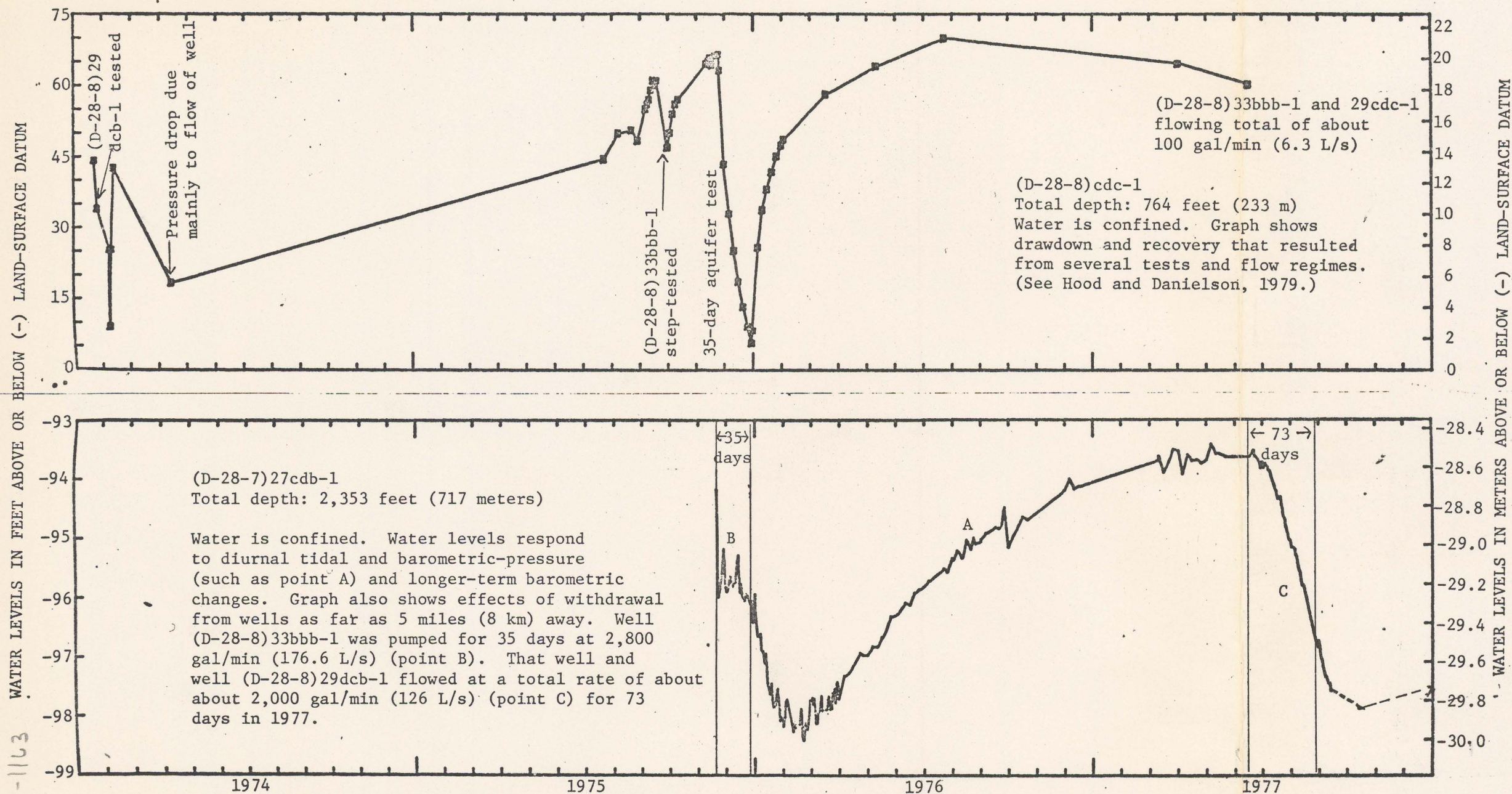
Figure 21.--Water levels in two wells finished in the Navajo Sandstone near Calneville, 1974-77.
