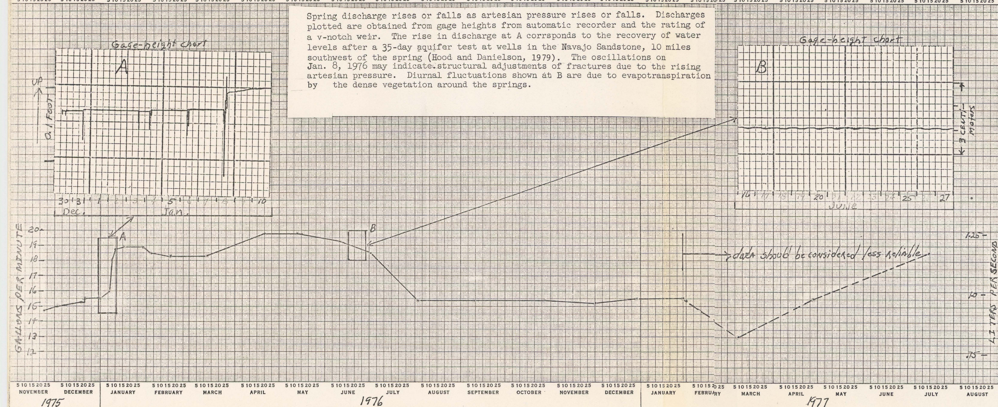
Figure 22.--Discharge of spring (D-27-8)12cca-S1, one of the Caine Springs.
