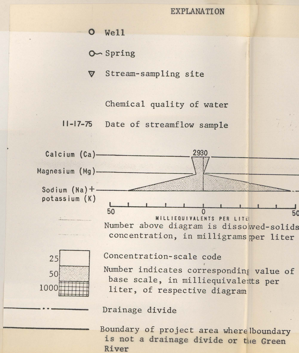
Figure 28.--Map showing chemical quality of surface inflow and outflow and of ground water in the Navajo Sandstone in the lower Dirty Devil River basin area, Utah.
