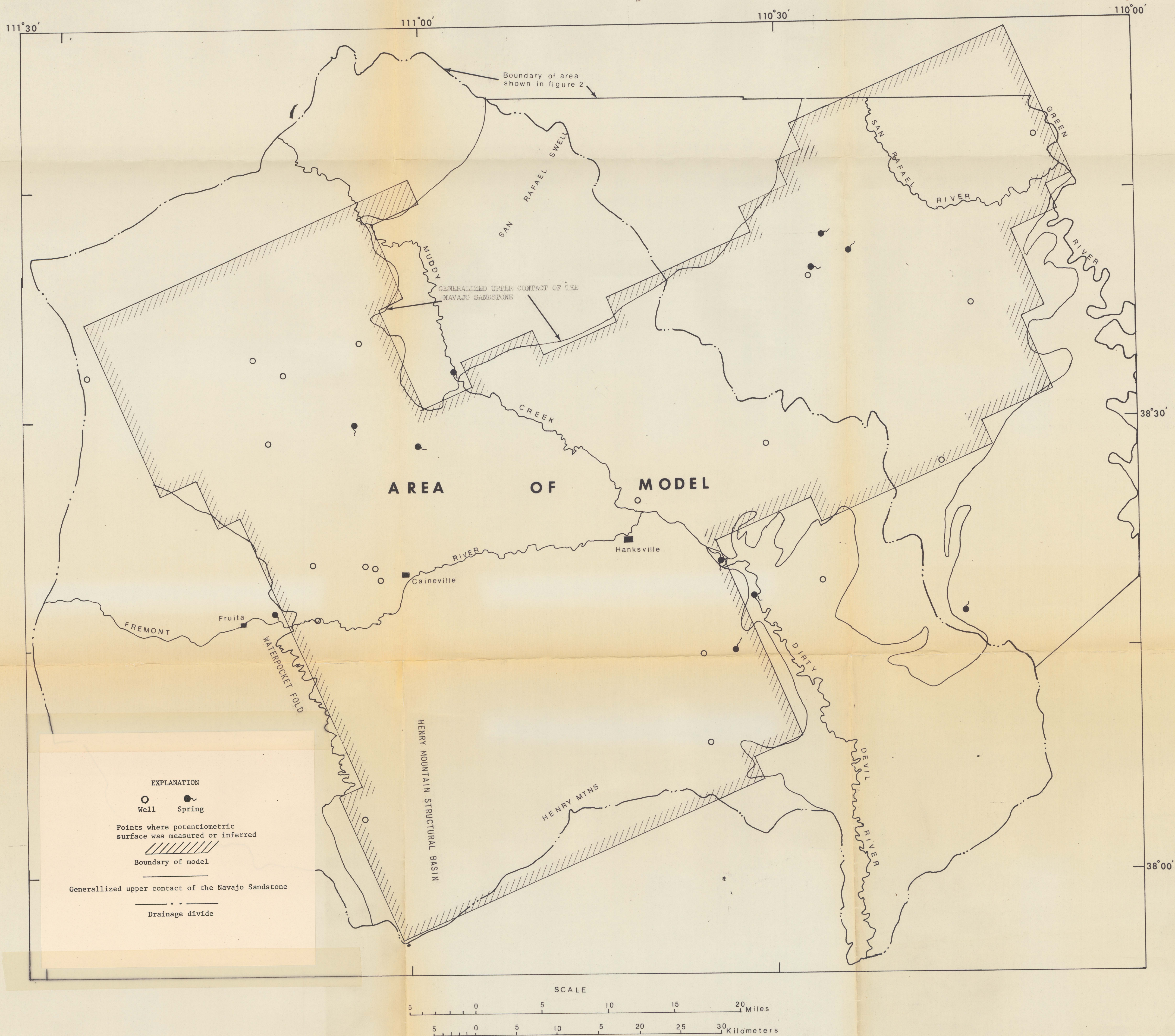
Figure 29.—Area of the digital model of the Navajo Sandstone aquifer.
