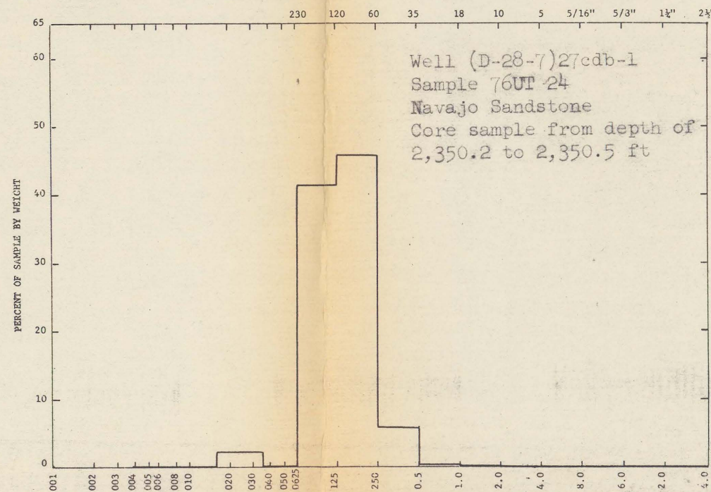
Figure 7.--Grain-size distribution in samples of the Navajo and Wingate Sandstones. (Left side of graph dashed where percentage of smaller grain-size fractions was not determined; see also tables 11 and 12 and Hood and Danielson, 1979, tables 2 and 3.)
