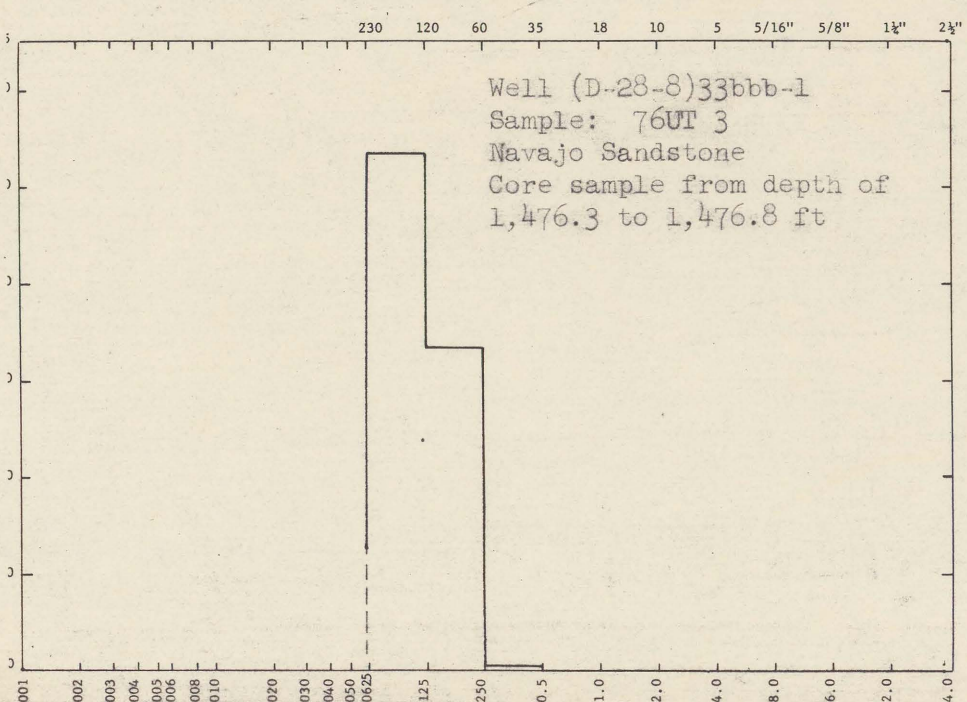
Figure 7.--Grain-size distribution in samples of the Navajo and Wingate Sandstones. (Left side of graph dashed where percentage of smaller grain-size fractions was not determined; see also tables 11 and 12 and Hood and Danielson, 1979, tables 2 and 3.)
