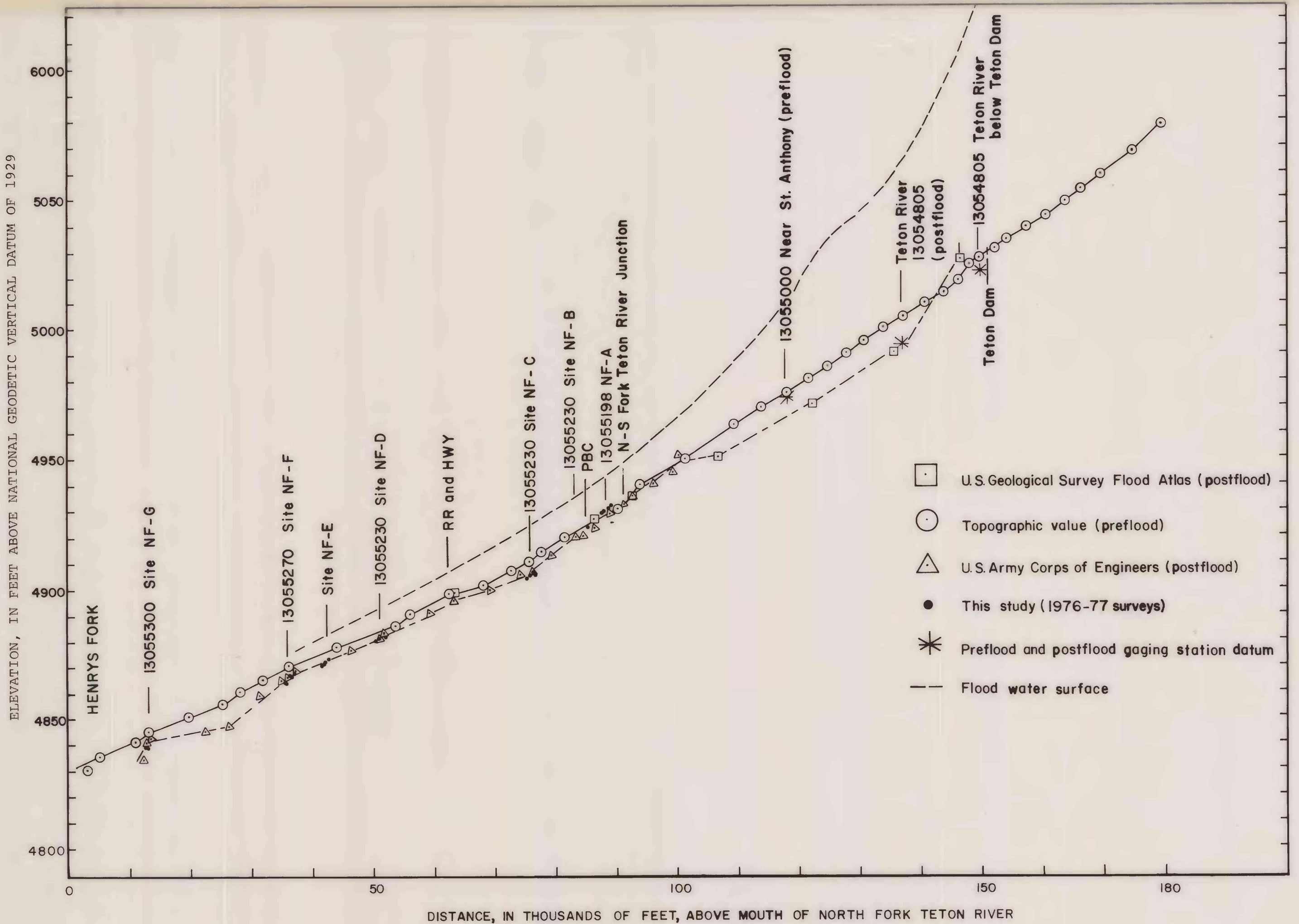
Figure 7. Streambed profile below Teton Dam site (preflood and postflood).
